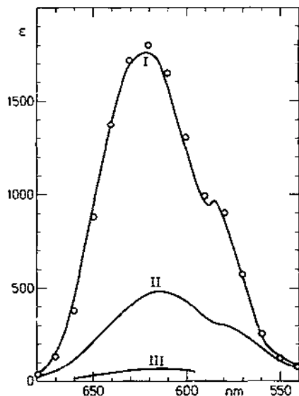
Fig. 4. Curve I, absorption spectrum ( \epsilon vs. \lambda ) of \text{H}_2\text{Co}(\text{NCS})_4 in 2-octanone ( C_{\text{Co(II)}} = 0.000412 ) prepared by extraction from a 5 M \text{NaNCS} , 0.05 M acid cobalt(II) solution. The open circles indicate the nearly identical spectrum probably of \text{Na}_2\text{Co}(\text{NCS})_4 , in 2-hexanone ( C_{\text{Co(II)}} = 0.000249 M) prepared by extraction from a similar \text{Co}(\text{NO}_3)_2 - \text{NaNCS} solution but without added \text{HNO}_3 . Curve II, spectrum of [\text{Co}(\text{NCS})_4]^{2-} in 10.6 M aqueous \text{NaNCS} . Curve III, estimated spectrum of [\text{Co}(\text{NCS})_3\text{H}_2\text{O}]^- in aqueous solution.
